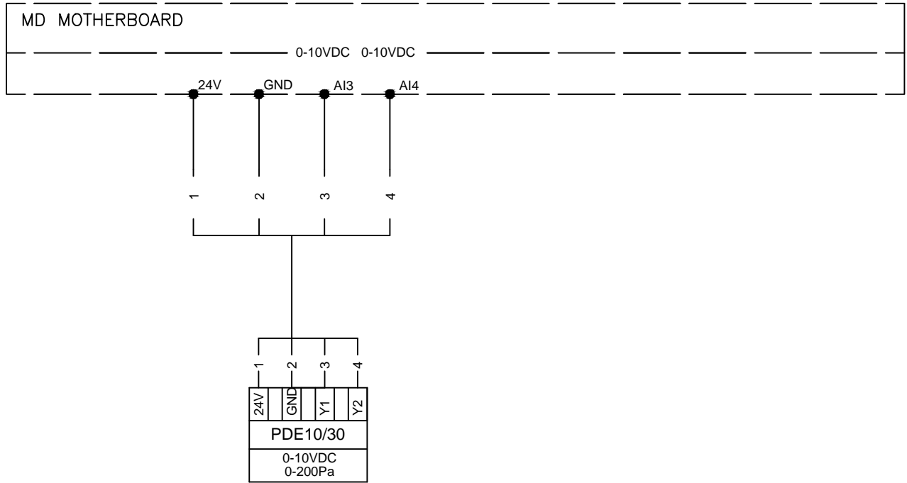
SUPPLY AND EXTRACT AIR DUCT PRESSURE MEASUREMENT, DUAL DIFFERENTIAL PRESSURE TRANSMITTER
