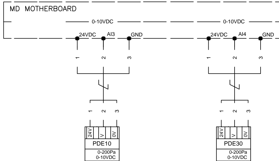
SUPPLY AIR DUCT PRESSURE MEASUREMENT, DIFFERENTIAL PRESSURE TRANSMITTER
