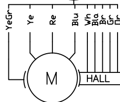
HRW MOTOR XFM605G-A20
